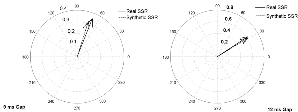
FIGURE 4.10 12ms gap phase and magnitude plot of both real and synthetic ASSRs (Right). 9ms gap phase and magnitude plot of both real and synthetic ASSRs (Left).
